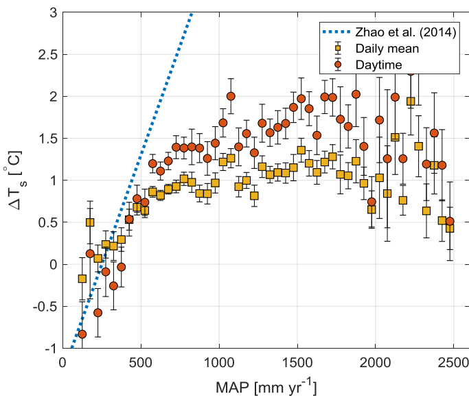
Fig 1: Urban-rural surface temperature difference ( \Delta T_s ) as a function of mean annual precipitation (MAP). Binned data are presented by mean \pm SEM. The linear relation proposed by Zhao et al. (2014) is also plotted for reference.
