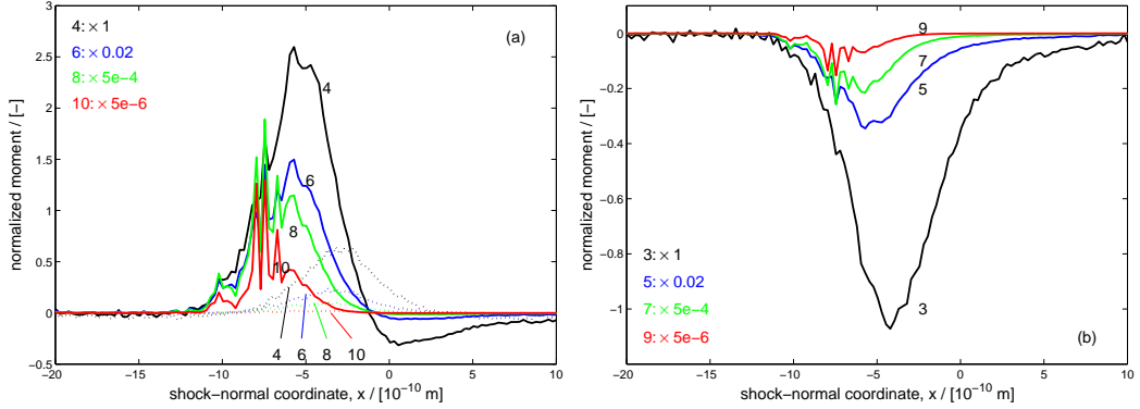
Figure 3: Even (a, left) and odd (b, right) moments of the velocity distribution function for a shock wave in dense nitrogen. The labels indicate the order of the moment. The solid lines are for the molecular velocities in shock-normal direction, the dotted lines for velocities within the shock plane. The odd moments for the shock-parallel velocities are zero (within the measurement uncertainty) and are not shown. The curves are scaled to fit in the same axes. The scaling factors, which have been applied for each order, are shown in each panel.
