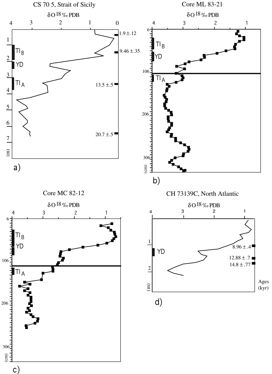
Fig. 9. \delta^{18}\text{O} (smoothed) of G. bulloides from cores ML 83-21 (b) and MC 82-12 (c), compared with \delta^{18}\text{O} (a) from core CS 70 5 from Strait of Sicily (Vergnaud-Grazzini et al. , 1988) and \delta^{18}\text{O} (d) from core CH 73139C from North Atlantic (Duplessy et al. , 1981).
