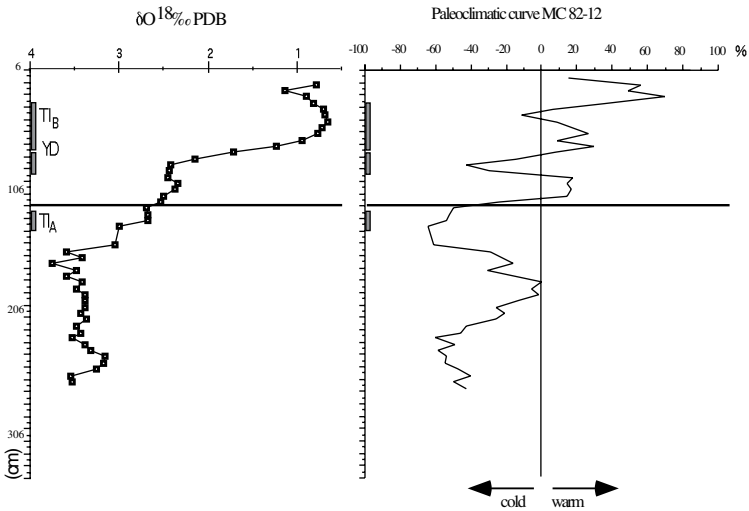
Fig. 12. – Oxygen stable isotope curves of G. bulloides and paleoclimatic curves from cores ML 83-21 (a) and MC 82-12 (b).
