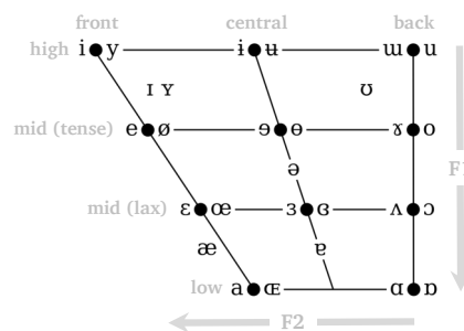
Figure 3: Vowel Chart
