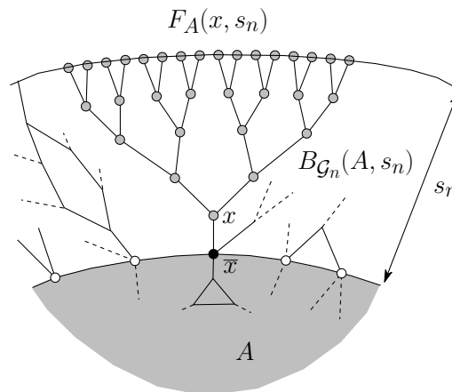
Figure 1: (adapted from [8]) The point x \in \partial_{\mathcal{G}_n} A is a good vertex at the boundary of A , the points in F_A(x, s_n) are marked grey.
