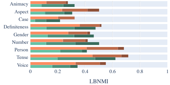
Figure 3: Comparison of per-attribute average lower-bound normalized mutual information (LBNMI) for fastText and BERT. Each bar is broken up into three components, which denote the LBNMI after selecting 2, 10 and 50 dimensions.
