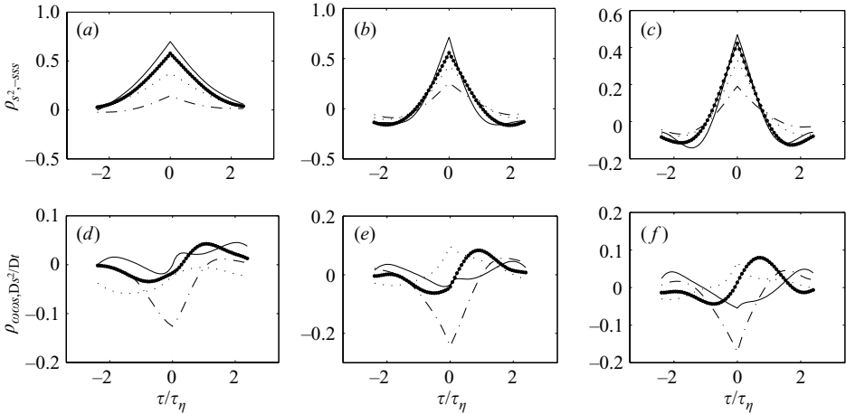
FIGURE 10. Lagrangian cross-correlation functions \rho_{s^2, -sss} and \rho_{\omega_s, Ds^2/Dt} for conditioned trajectory samples: high-strain–low-entropy (—), high-strain–high-entropy (–•–•–), high-entropy–low-strain (· · ·), low-entropy–low-strain (– · – ·). Correlations are computed following the three procedures: (a, d) \rho_{XY}(\tau) , (b, e) \bar{\rho}_{XY}(\tau) , (c, f) \hat{\rho}_{XY}(\tau) .
