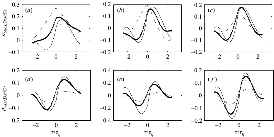
FIGURE 11. Lagrangian cross-correlation functions \rho_{\omega_s, D\omega^2/Dt} and \rho_{-sss, Ds^2/Dt} for conditioned trajectory samples: high-strain–low-entropy (—), high-strain–high-entropy (–•–•–), high-entropy–low-strain (· · ·), low-entropy–low-strain (– · – ·). Correlations are computed following the three procedures: (a, d) \rho_{XY}(\tau) , (b, e) \bar{\rho}_{XY}(\tau) , (c, f) \hat{\rho}_{XY}(\tau) .
