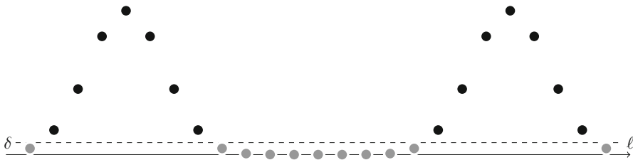
Fig. 4 The function f_\lambda^+ from the introduction after discretisation. Entries of the resulting signal that fall below a certain threshold \delta > 0 are coloured in grey. The remaining entries are coloured in black and make up the vertex set V_\delta . In this picture, we can clearly see the two temporal islands
