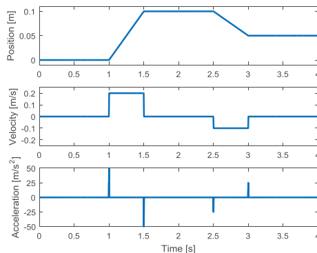
Fig. 2. 1-dimensional positioning.
