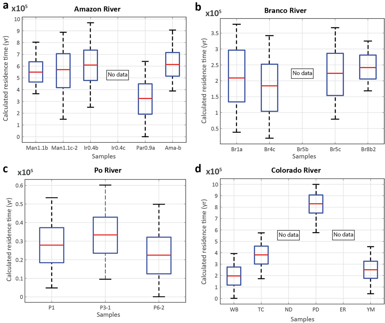
Figure 3. Boxplots of calculated residence times from the four examined rivers. Each box presents all calculated residence times for 1,000 runs, with a maximum of 10^6 steps and a maximal run time of 10^6 yr (see specific river parameters in Table 1). The central red mark is the median, and the bottom and top blue edges of the box indicate 25th and 75th percentiles, respectively. The dashed whiskers extend to the most extreme data points, which are not considered outliers (the presented data set does not contain outliers).
