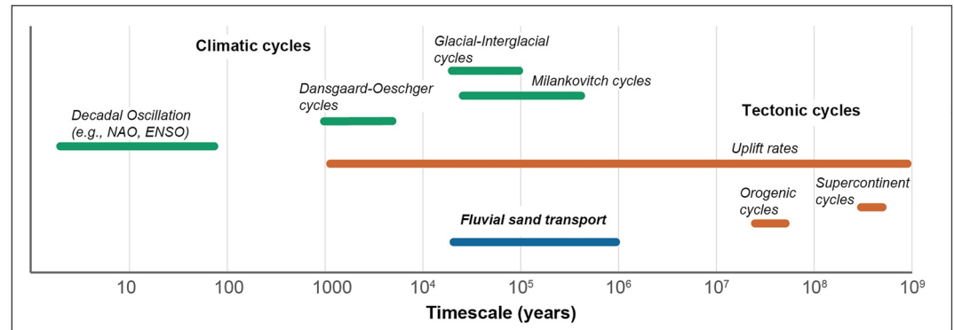
Figure 5. A comparison of timescales of fluvial transport and major tectonic and climatic variations. Timescales of fluvial transport represent sediment residence times in large rivers reported here as well as published lag times and sediment storage from large rivers across the globe (Blöthe & Korup, 2013; Clift & Giosan, 2014; Fülöp et al., 2020). Climatic cycles are after Foreman and Straub (2017). ENSO stands for El Niño–Southern Oscillation, and NAO stands for North Atlantic Oscillation. Tectonic cycles are after Meade (1994). The timescales of fluvial transport are longer or similar to climatic variations and mostly shorter compared to tectonic variations, implying that climatic variations and short-term tectonic events will be buffered by the fluvial transport system and will not be preserved in the sedimentary record.
