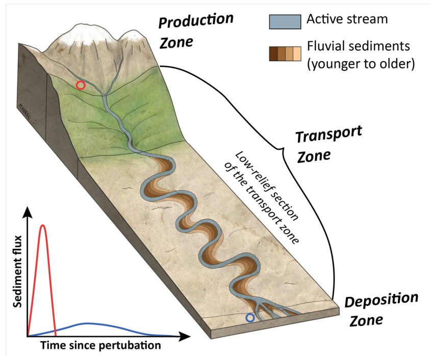
Figure 1. Schematic diagram of sediment transport in large-scale fluvial systems. Sediment is mainly produced in the mountainous region upstream (the Production Zone) and is transported to the depositional basin (Deposition Zone). As sediments reach the downstream low-relief section of the transport zone, they are intermittently deposited at floodplains and channel bars for varying periods and depths represented here by shades of brown. Storage in a specific point in space occurs until an erosional process remobilizes and transports the sediment further downstream. These continuous cycles of erosion and deposition lead to a complex storage framework of sediment within the fluvial system and make it difficult to quantify the transport time of sediments in rivers. The graph on the bottom left shows changes in sediment flux as a function of time (after Straub et al., 2020). The perturbation in sediment flux due to climate-induced increase in erosion rates at the production zone (red) is buffered when the signal reaches the deposition zone (blue) because of the residence times of sediment in the low-relief section of the transport zone.
