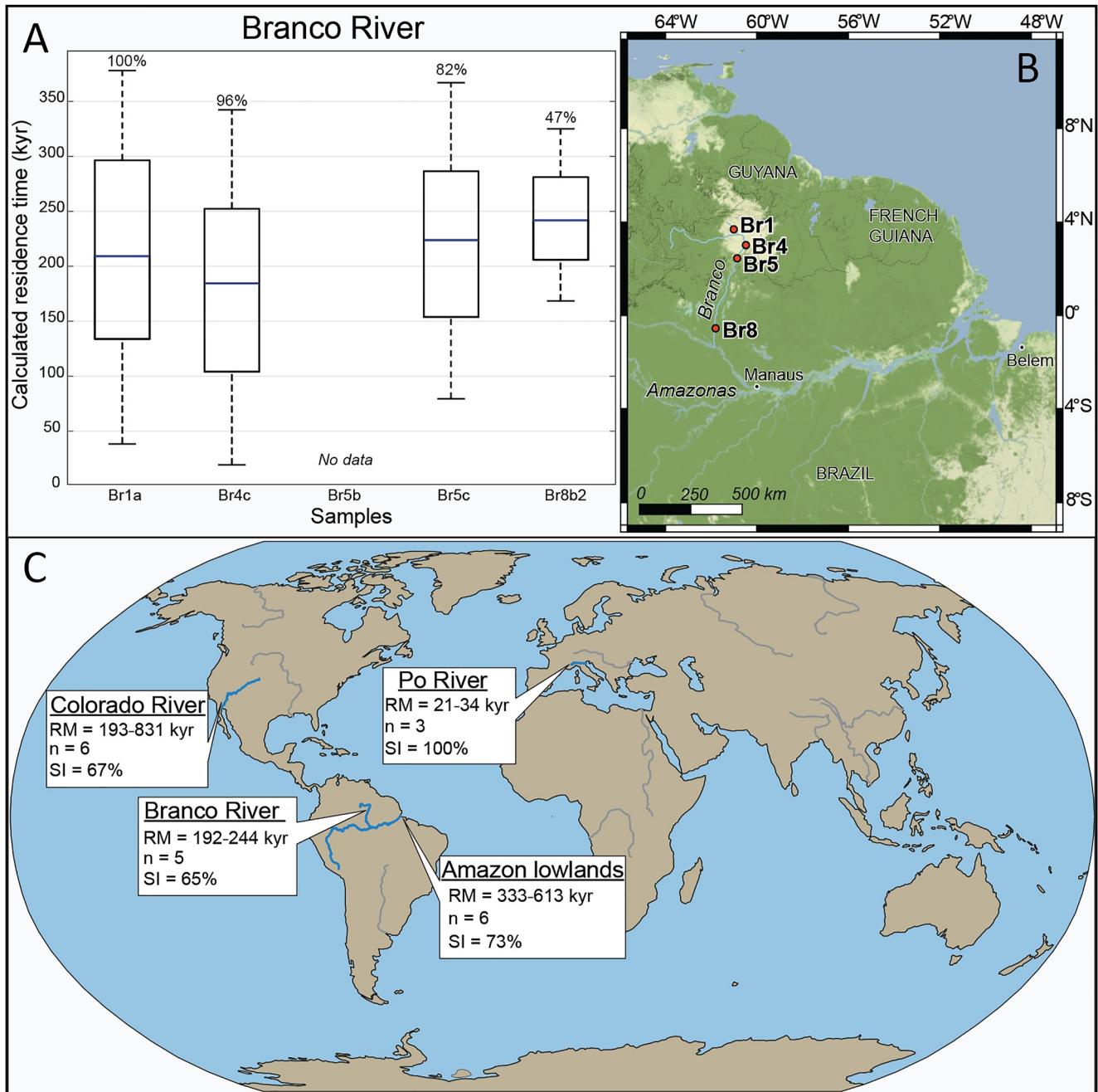
Figure 4. The residence time of sand-sized silicate sediments in large rivers. (a) Box plot of calculated residence times and percentage of successful runs for each sample in the Branco River. (b) Map of the corresponding sampling stations along the Branco River. (c) Map showing the locations of the rivers analyzed in this work and the model results. Sediment residence time is presented as the range of medians (RM) calculated for each sample in a specific river. n , number of samples analyzed, and SI is the averaged success rate from all stations.
