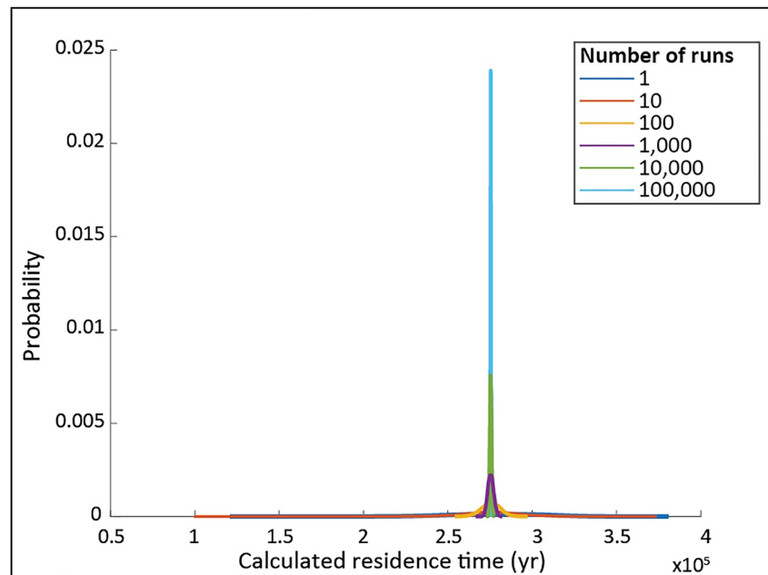
Figure 2. Sensitivity of the model to the number of runs. Probability of the maximal calculated residence time from 1 to 10^5 model runs for sample CRWB (Colorado River) with burial depth 10 m and burial time 100 years. The spread of residence time of 1,000 runs (purple) is smaller than the natural analytical uncertainty calculated from cosmogenic nuclide concentrations (see Table S1 in Supporting Information S1), allowing for a reliable calculation of residence times. This test was applied for all rivers and produced similar results.
