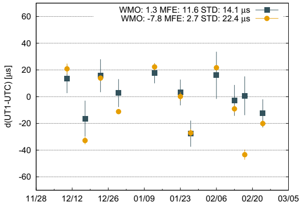
(a) Time series of the d(UT1-UTC) estimates between VG1 (blue squares) and VG2 (yellow, circles).
