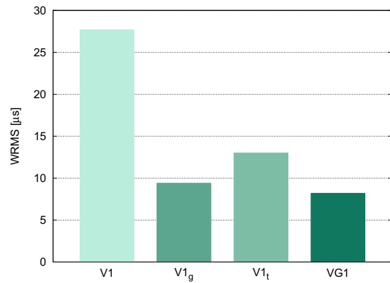
(a) The WRMS differences of VG1, V1, and its augmentations with gradients ( V1_g ) and the complete troposphere set ( V1_t ) with respect to the VG2_{3c+} solution.
