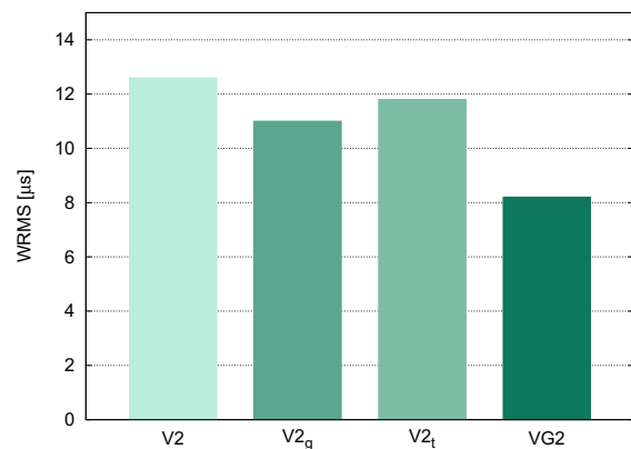
(b) The WRMS differences of VG2, V2, and its augmentations with gradients ( V2_g ) and the complete troposphere set ( V2_t ) with respect to the VG1_{3c+} solution.
