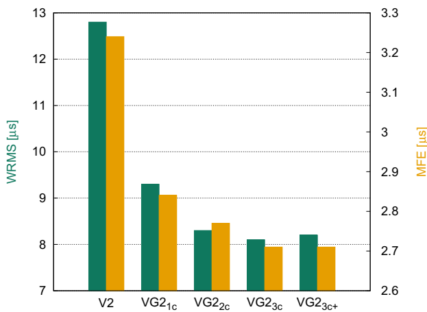
Fig. 8 The impact of the incremental addition of GNSS constellations to V2 in terms of WRMS differences with respect to the VG1_{3c+} solution (WRMS, green) and mean formal error (MFE, yellow)
