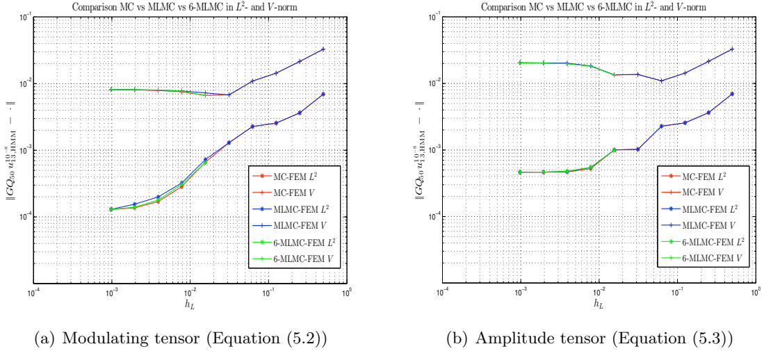
FIGURE 3. Estimated L^2(\Omega; L^2(D)) -errors and L^2(\Omega; V) -errors with respect to the homogenized solution \mathbb{E}[\bar{u}] of Finite Element based methods for the modulating and the amplitude tensor.
