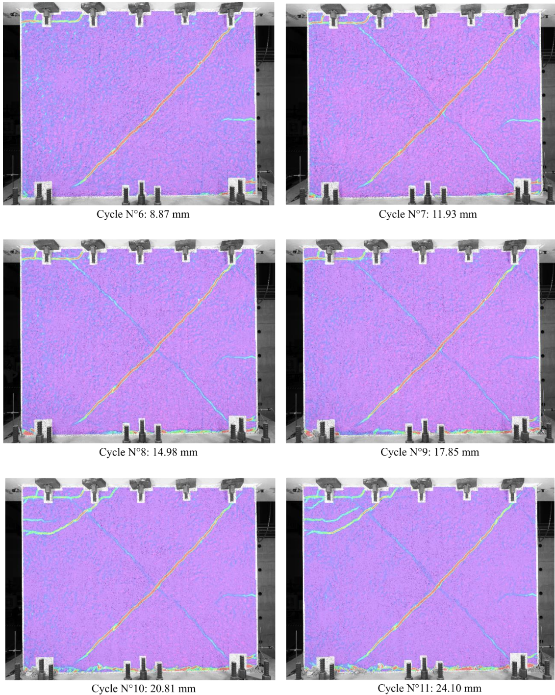
Figure 4: DIC displacement fields, showing the transition between shear and sliding.
