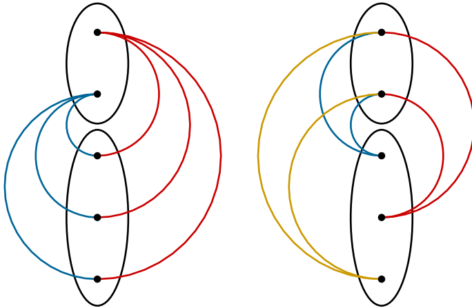
Fig. 2 The partitions of a p^* into \gamma_0^p, \gamma_1^p on the left and into \beta_0^p, \beta_1^p and \beta_2^p on the right
