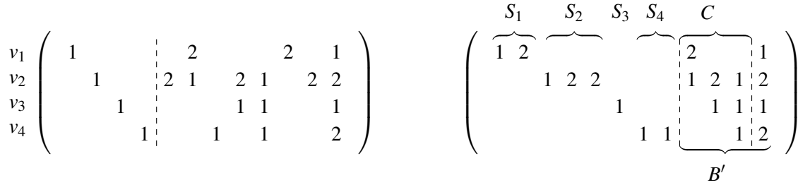
Figure 1: On the left, a matrix M over \mathbb{F}_3 , where blank entries denote 0. On the right, we rearranged the columns of M for better visualization.
