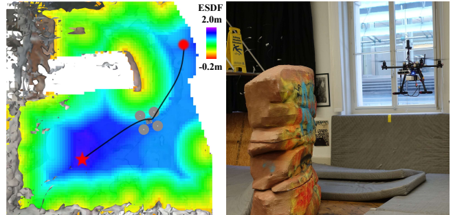
Fig. 1: Real-world mapping and path planning experiment. A Micro-Aerial Vehicle (MAV) is tasked to navigate towards a goal position, while avoiding the obstacle visible on the right. Voxfield generates the ESDF map visible on the left onboard the MAV in real time, which is used for planning. The red dot and the star are the starting and goal position, respectively.
