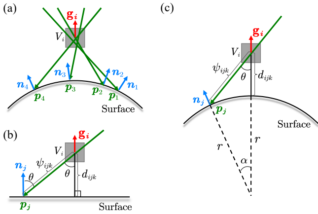
Fig. 3: Non-projective TSDF calculations for voxel V_i : the updated voxel is represented in grey, rays from raycasting in green, the surface normals in blue and the field gradient in red. (a) shows the integration of voxel V_i 's TSDF-gradient by taking a weighted average of the normals on the surface point hit by the rays cast through V_i from different sensor positions. (b) and (c) show the geometric relationship between the projective distance \psi_{ijk} and the non-projective distance d_{ijk} under the assumption of a flat or curved surface, respectively. The radius of the curved surface in (c) is marked as r .
