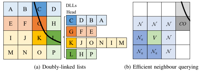
Fig. 4: Diagram of Voxfield's ESDF algorithm simplified in 2D: (a) the black line represents the surface, the saturated voxels (C, G, K, L) are occupied while the other voxels are free or behind the surface. Each of the doubly-linked lists has an occupied voxel as the head node. The other nodes in the list are the voxels where the head node is the closest occupied voxel. (b) the voxels in grey are occupied. We are querying the neighbouring voxels \mathcal{N} of the voxel V . The subset of neighbouring voxels affected by a change of V , namely voxels \mathcal{N}_g , can be identified from the neighbourhood based on the direction of the closest occupied voxel CO of V .
