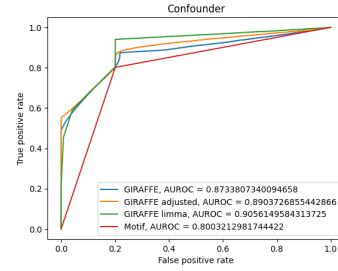
Figure 5.9: ROC curves for Figure 5.6
