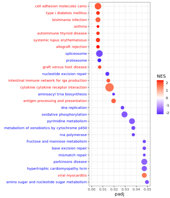
Figure B.10: Pathways enriched for healthy lung using PANDA.
