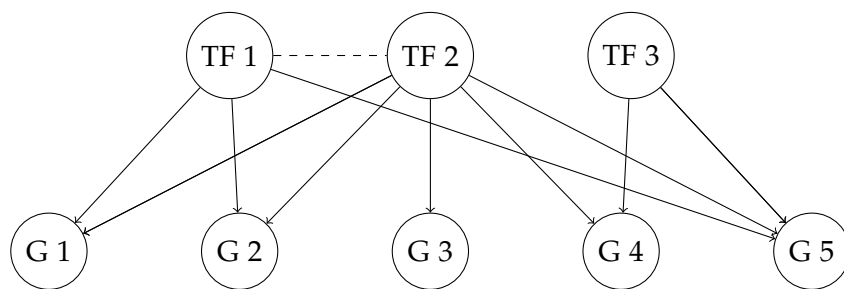
Figure 4.2: Abstract representation of the gene regulation machinery. The dashed edges between transcription factors represent protein protein interactions and are given as prior knowledge. We estimate the regulatory interactions as directed edges from transcription factors to genes.
