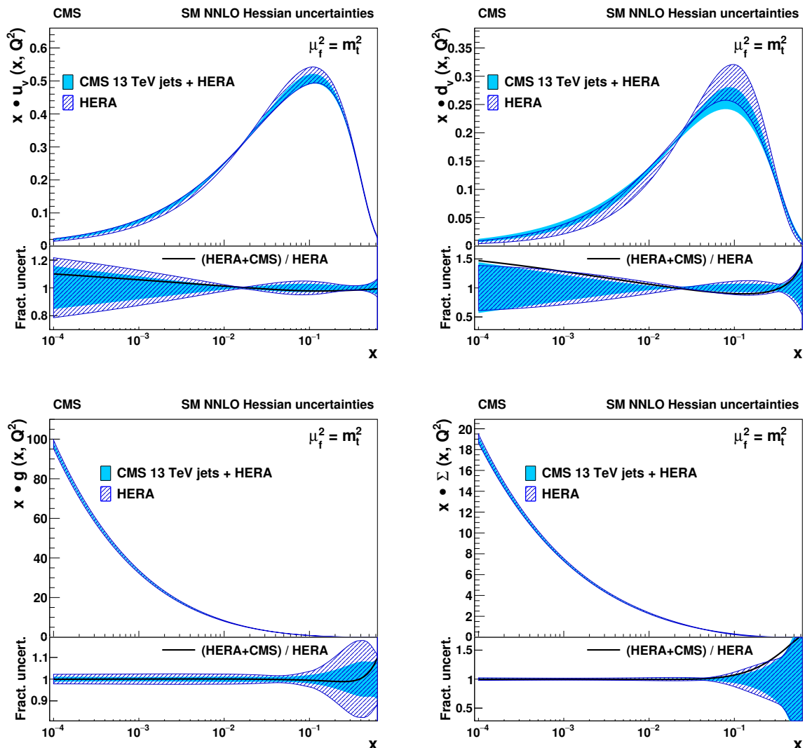
Figure 3. The u-valence (upper left), d-valence (upper right), gluon (lower left), and sea quark (lower right) distributions shown as a function of x at the scale \mu_f = m_t . The filled (hatched) band represents the results of the NNLO fit using HERA DIS and the CMS inclusive jet cross section at \sqrt{s} = 13 TeV (using the HERA DIS data only). The PDFs are shown with their total uncertainty. The prediction for the inclusive jet cross section is obtained using NNLO interpolation grids. In the lower panels, the comparison of the relative PDF uncertainties is shown for each distribution. The line corresponds to the ratio of the central PDF values of the two variants of the fit.
