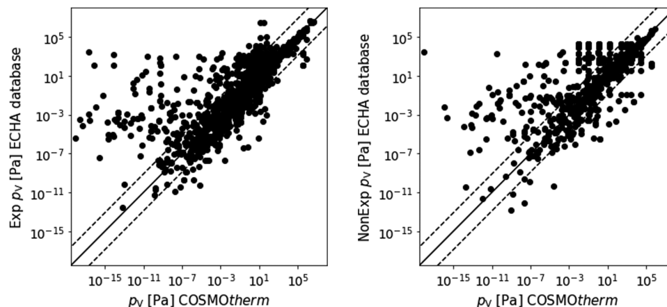
FIG. 7. Comparison of the experimental (left) and non-experimental (right) vapor pressure from the ECHA database with no qualifier or qualifier “ca.” with the data from COSMOtherm for neutral organic substances with one component (full registrations and NONS). The solid line is the 1:1 line, the dashed lines indicate a deviation of 1.9 orders of magnitude. COSMOtherm values refer to 20 °C, values from the ECHA database to (20 \pm 5) °C.
