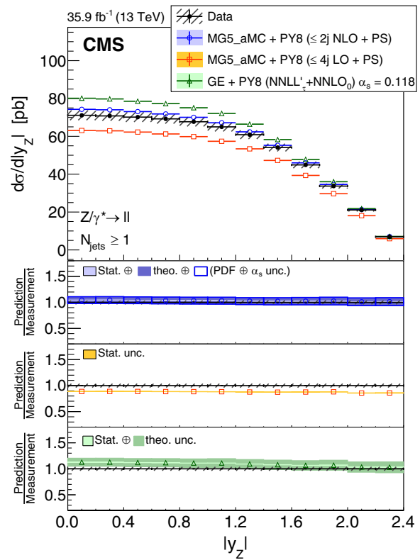
FIG. 12. The measured differential cross section as a function of Z boson |y| for events with at least one jet. Details on the presentation of the results are given in Fig. 4.
