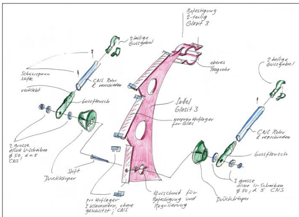
Figure 2. Construction sketch of the “CLA” façade by Fosco Fosco-Oppenheim Vogt Architects
