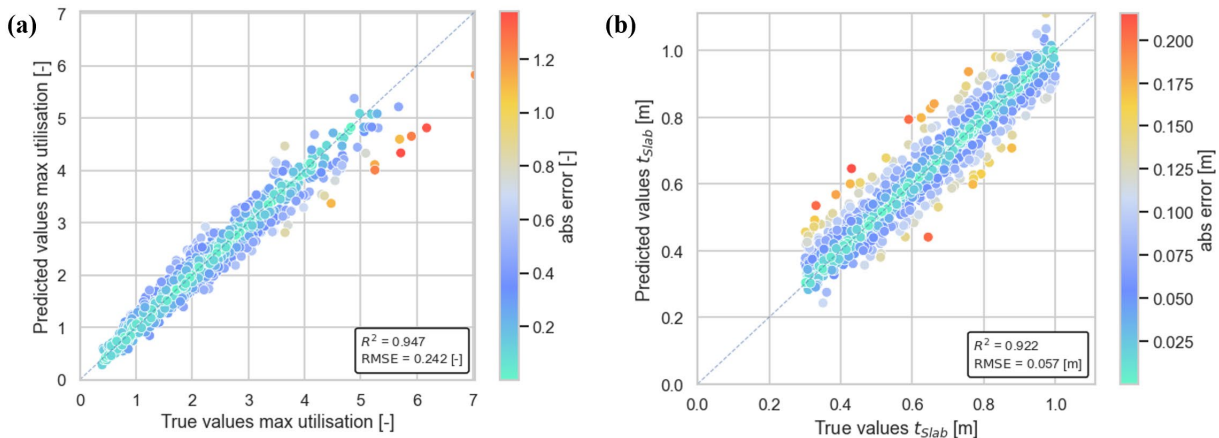
Figure 6: Performance on test set: (a) Forward (surrogate) model predicting max. utilisations, (b): Inverse (generative) model generating suitable deck slab thicknesses.
