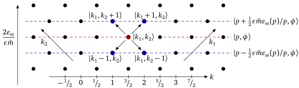
Figure 2: Discrete states |k_1, k_2\rangle of AdS irrep vs. continuous states |p, \phi\rangle of Poincaré irrep. Note that the lattice of permissible k is alternating between integers and half-integers for consecutive energy levels.
