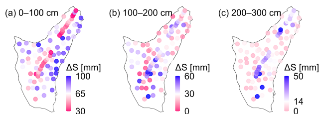
Figure 10. Spatial pattern of annual soil moisture storage change ( \Delta S ) integrated over depths of (a) 0–100 cm, (b) 100–200 cm, and (c) 200–300 cm. In the top 100 cm of the soil profile (a), soil moisture changes are much greater on the hillslopes than in the gully and greater on the NW-facing slope than on the SE-facing slope. These differences become less distinct between 100 and 200 cm (b) and become almost indistinguishable below 200 cm (c), where instead the greatest soil moisture changes occur in the gully. Note that the color scales differ among the three panels. Blue colors indicate changes that are larger than the catchment average; red values indicate changes that are smaller than the catchment average.
