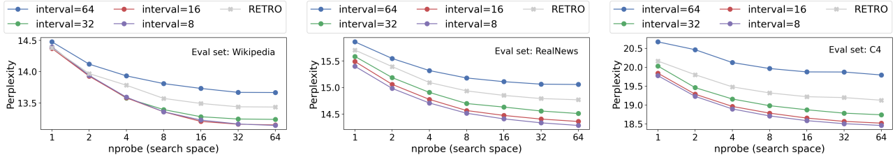
Figure 5. Perplexity of retrieval-augmented generation when applying various retrieval intervals and search space configurations ( nprobe ).
