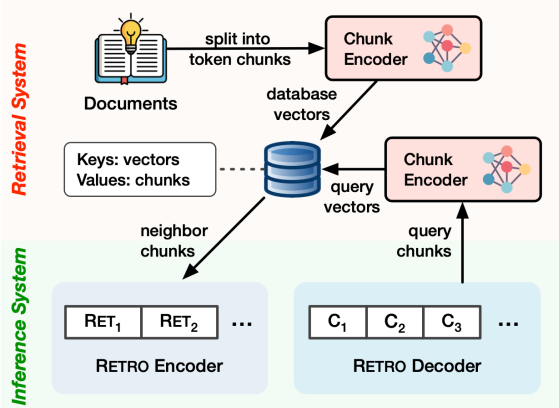
Figure 2. Retrieval-augmented generation with RETRO.
