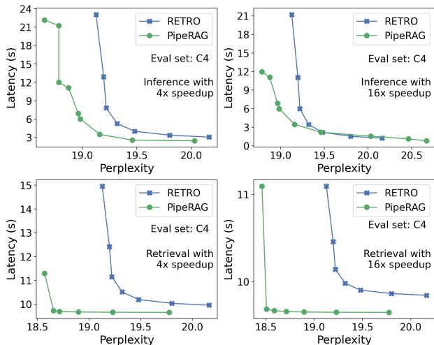
Figure 7. Trends in PipeRAG efficiency when deployed on future hardware that enables faster retrieval or inference.
