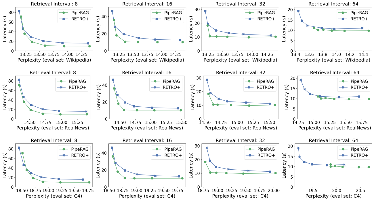
Figure 10. The latency-perplexity comparison between PipeRAG versus RETRO given the same retrieval intervals.
