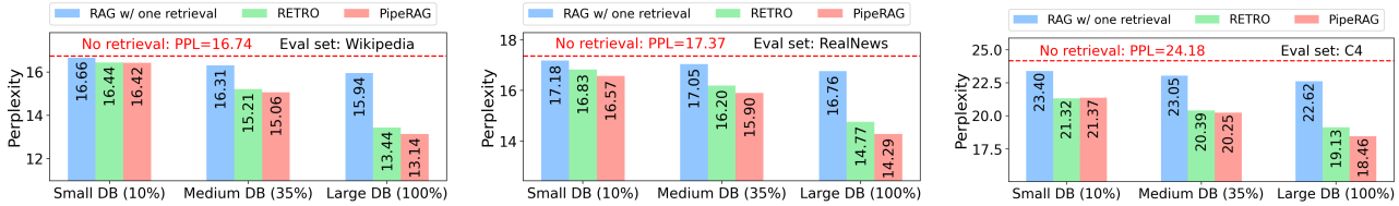
Figure 4. The effect of database sizes and retrieval strategies on language modeling perplexity (lower perplexity means higher quality).
