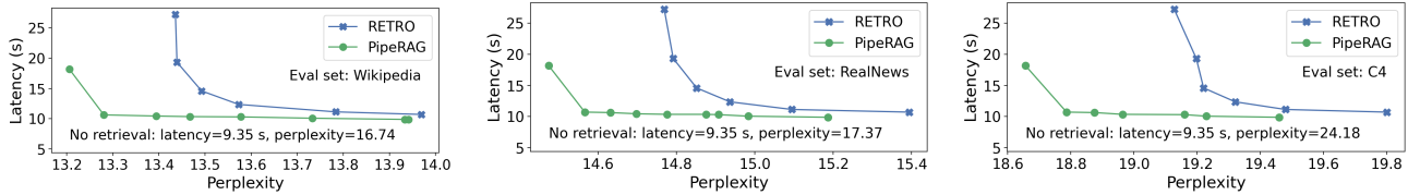
Figure 6. PipeRAG significantly outperforms RETRO on the latency-perplexity Pareto frontier (lower latency and perplexity are better).
