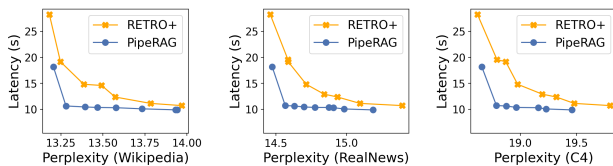
Figure 8. Even if the baseline model supports flexible retrieval intervals (RETRO+), PipeRAG still significantly outperforms it in efficiency thanks to the proposed pipeline parallelism.
