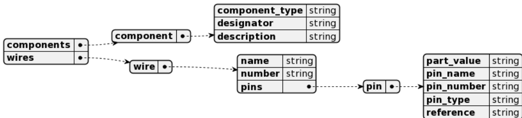
Figure 2.1: Illustration of the schema of the netlist from Enzian.
