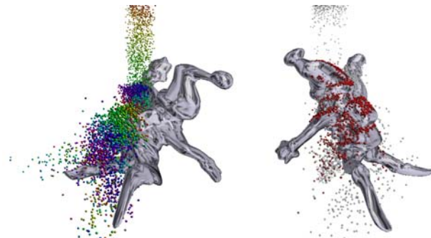
Figure 12: Deforming Santa and particles. Red color on the right-hand side indicates actual or recent contact.
