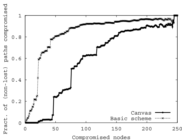
Figure 3: Canvas compared to a basic trust-chain approach
