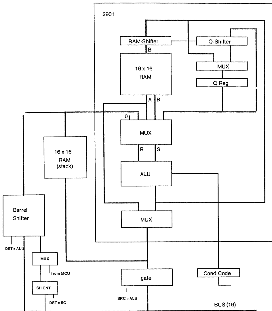
Fig. 12. The Arithmetic-Logic Unit
