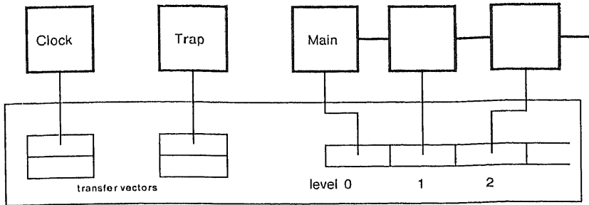
Fig. 5. The three processes of Medos
