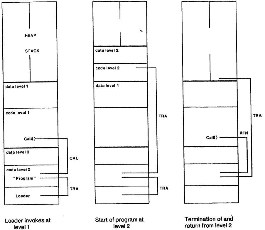
Fig.2. Loading of program at level 2
