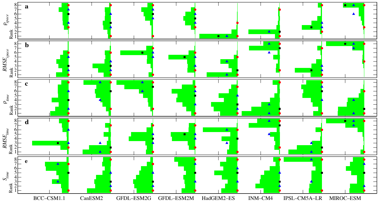
Figure 3. Skill rank by model. Histograms for ranked (a) spatial correlation, \rho_{space} ; (b) spatial RMSE, RMSE_{space} ; (c) temporal correlation, \rho_{time} ; (d) temporal RMSE, RMSE_{time} ; and (e) distributional similarity, S_{time} . Lower ranks denote relatively higher levels of model–data agreement. Distributions are displayed as horizontal histograms and share the same scale within each panel. Colored symbols give percentiles. Median, black square; interquartile range (25–75 percentiles), blue triangles; and 2.5–97.5 percentiles, red circles. Some symbols jittered to avoid overlap.
