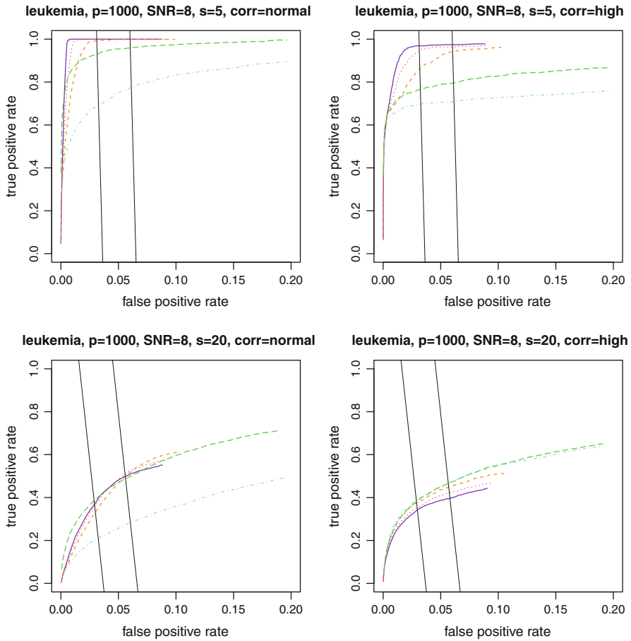
Fig. 4 Partial ROC-curves for Leukemia dataset with p = 1,000 , SNR = 8 : Lasso ( solid ), LENet ( dotted ), HENet ( dashed ), MER ( longdashed ) and SIS ( doidashed ). The oblique black lines represent the points in the TPR to FPR graphs where 0.5n ( left line ) and 0.9n ( right line ) variables are selected
