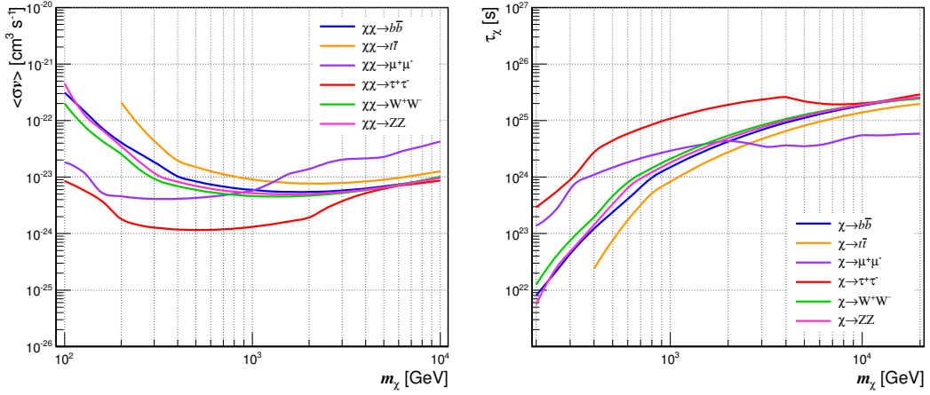
Figure 6. Upper limits on \langle\sigma_{\text{ann}}v\rangle ( left ) and lower limits on \tau_\chi ( right ), for secondary photons produced from different final state SM particles, from the Segue 1 observations with MAGIC.
