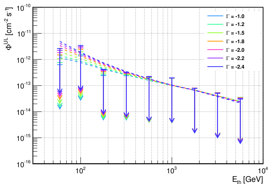
Figure 19. Integral flux upper limits from 157.9 hours of the Segue 1 observations with MAGIC, assuming a point-like source and a power law-shaped signal emission and different spectral slopes \Gamma . Dashed lines indicate the expectations for the null hypothesis case.
