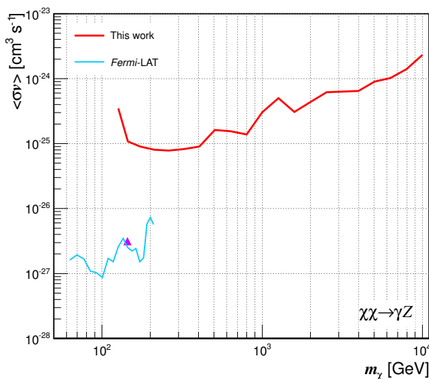
Figure 16. Upper limits on \langle\sigma_{\text{ann}}v\rangle for DM annihilation into a photon and a Z boson, from the Segue 1 observations with MAGIC (red line), compared with the exclusion curve from 2 years of the GC region observations with Fermi -LAT (blue line, [66]). Also show is the \langle\sigma_{\text{ann}}v\rangle value corresponding to the 130 GeV gamma-ray line (violet triangle, [64]).
