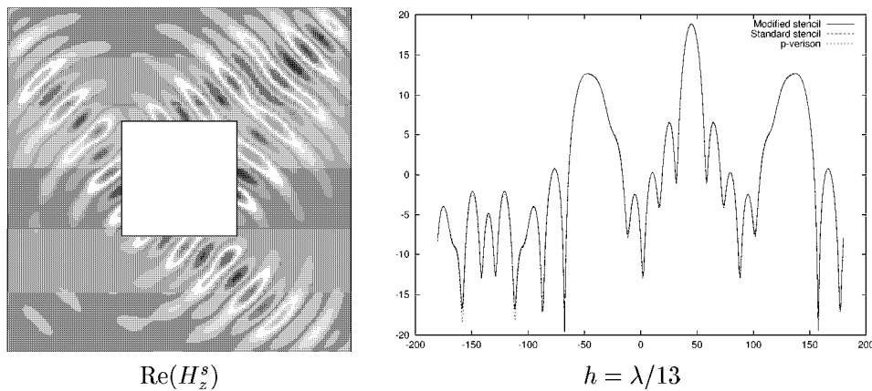
Figure 10: Scattering of plane wave by a PEC square of electrical length 3\lambda showing a contour plot of Re(H_z^s) and the scattering width distribution computed on a mesh with spacing h = \lambda/13 .
