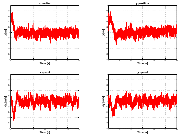
Fig. 6. Simulation: Integral backstepping position controller drives attitude controller in order to maintain the helicopter over a given point.
