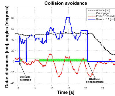
Fig. 9. Experiment: Collision avoidance with OS4. The helicopter flies back until the obstacle disappears.
