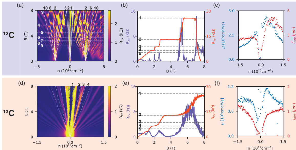
FIG. 2. Quantum transport measurement of ^{12}\text{C} (a),(b),(c) and ^{13}\text{C} (d),(e),(f) bilayer graphene. (a),(d) R_{xx} as a function of magnetic field B and carrier density n . White dotted tilted lines fit the Shubnikov–de Haas oscillations with filling factors shown in the figure. White dotted horizontal lines show the position at which the Brown-Zak oscillations appear. (b),(e) Example traces of the quantum Hall effect at n = 1.13 \times 10^{11} ( ^{12}\text{C} ) and n = 1.9 \times 10^{11} ( ^{13}\text{C} ). (c),(f) Carrier density n dependence of the mobility \mu and the mean free path l_{\text{mfp}} estimated from the low magnetic field data.
