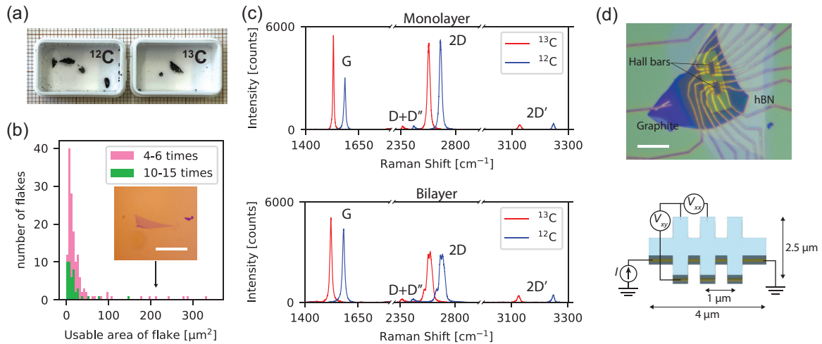
FIG. 1. (a) Optical picture of ^{12}\text{C} and ^{13}\text{C} graphite crystals. The minimum grid size in the background is 1 mm. (b) Histogram of ^{12}\text{C} graphene flake size. Inset shows a picture of the example bilayer flake. The scale bar is 50 \mu\text{m} . (c) Raman spectrum of ^{12}\text{C} and ^{13}\text{C} graphene. Top: monolayer graphene. Bottom: bilayer graphene. (d) Top panel: optical picture of the fabricated Hall bar. The scale bar is 10 \mu\text{m} . Bottom panel: schematic of the fabricated Hall bar.
