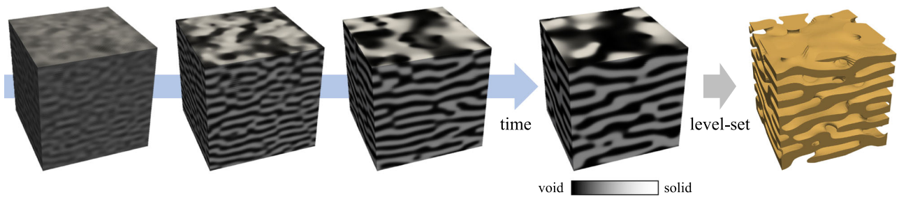
a Topology generation by simulating anisotropic spinodal decomposition
