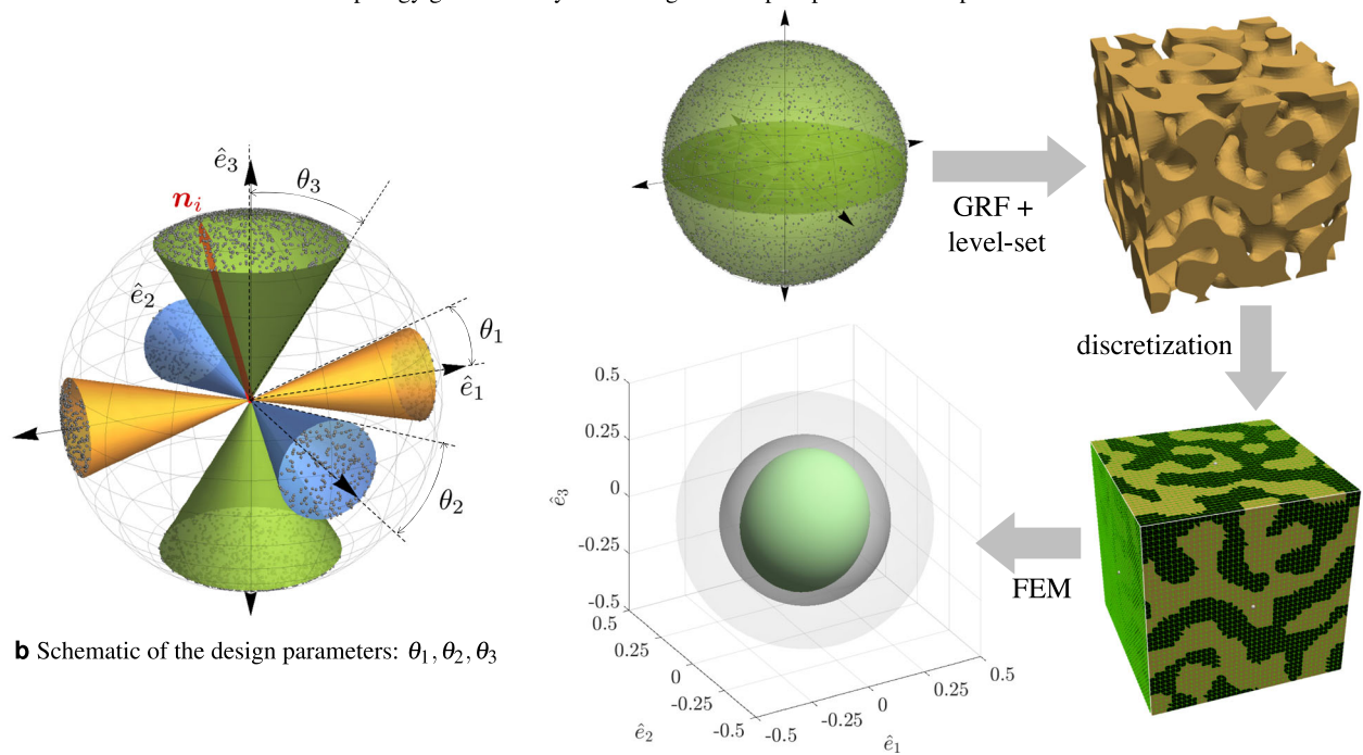
c Topology generation (via GRF) and computational homogenization
