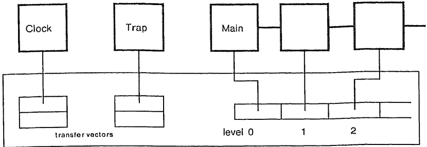
Fig. 5. The three processes of Medos
