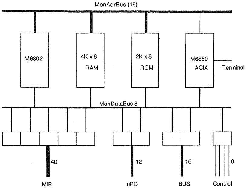
Fig. 19. Monitor with 6802 microprocessor
