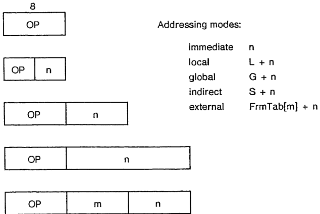
Fig. 8. Lilith instruction formats
