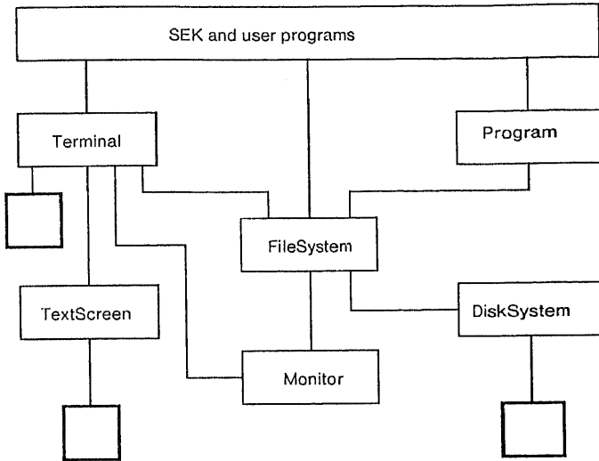
Fig. 6. Procedure call hierarchy
