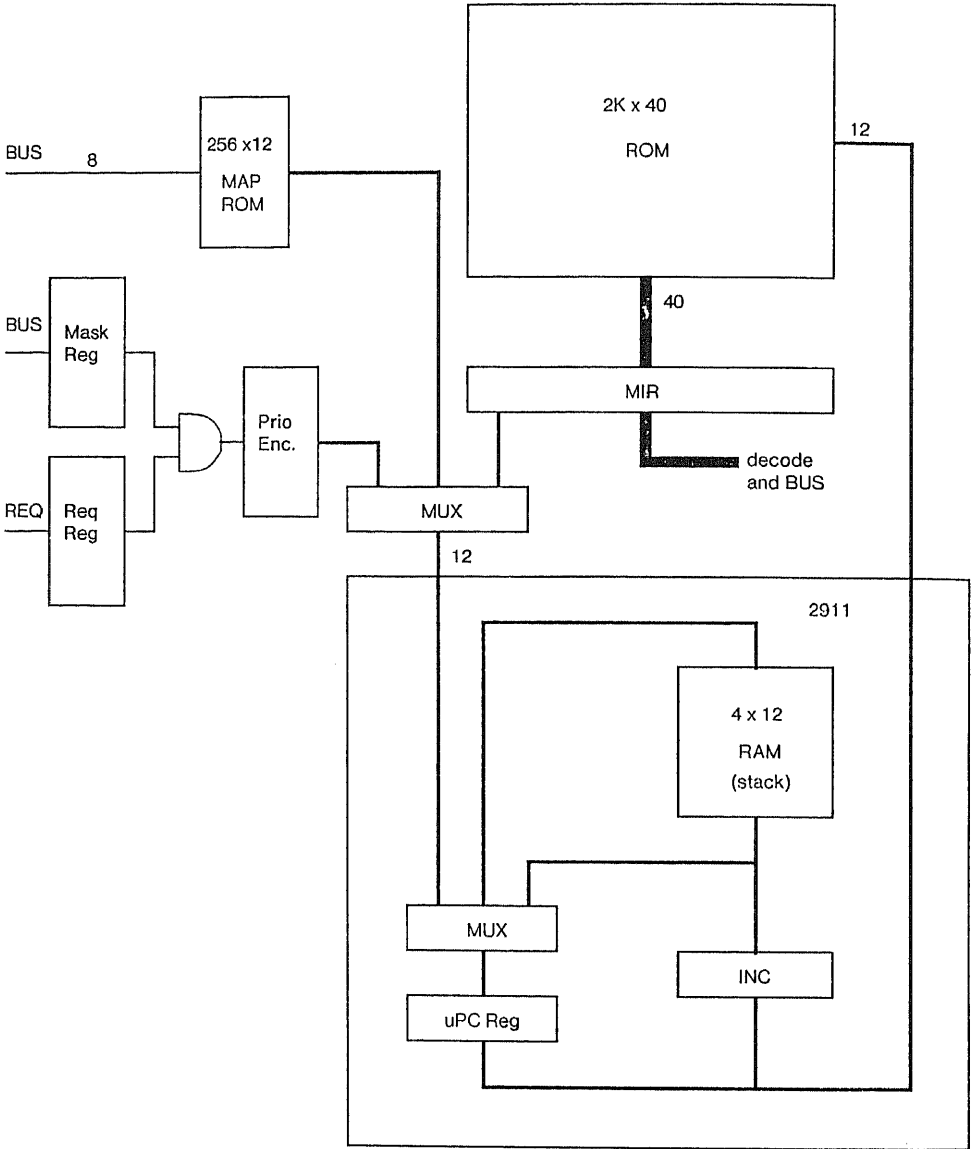
Fig. 11. The Micro-Control Unit
