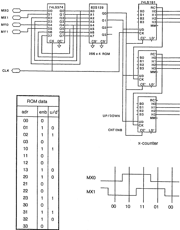
Fig. 18. The Mouse interface with x-counter
