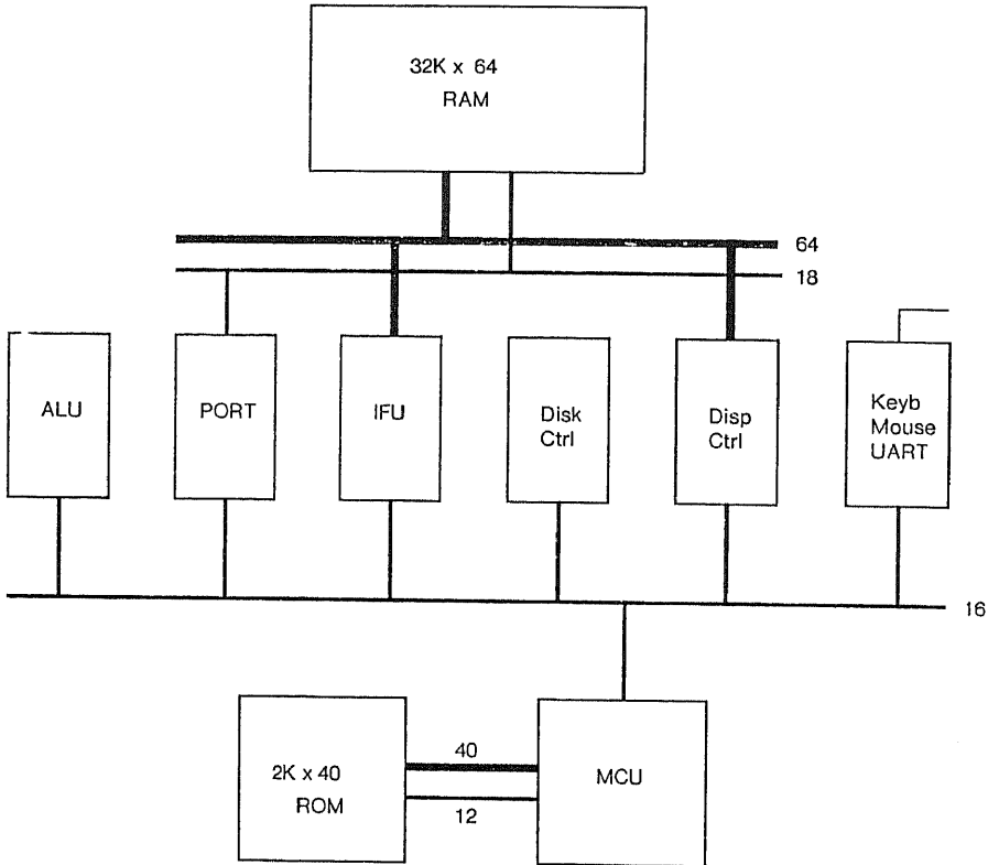
Fig. 9. Lilith hardware structure
