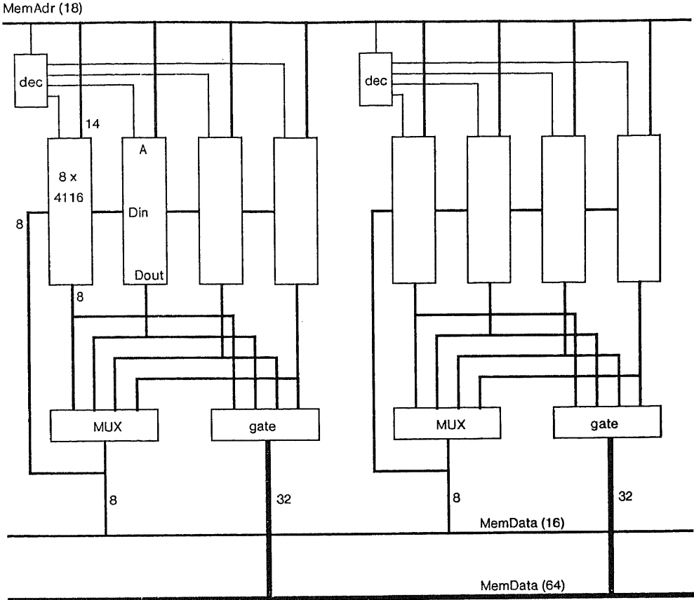
Fig. 14. Memory organization
