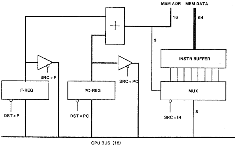
Fig. 17. The instruction fetch unit
