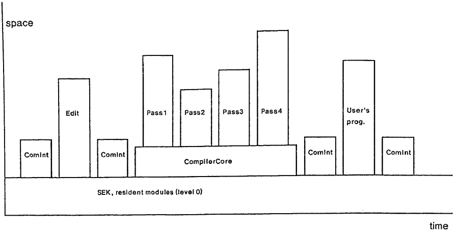
Fig.3. Typical sequence of program loadings
