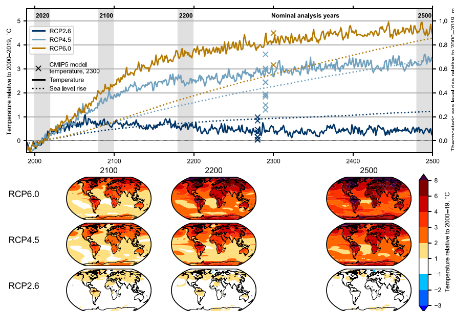
FIGURE 1 Top panel: Global mean near-surface air temperature (solid lines) and thermosteric sea-level rise (dotted lines) anomalies relative to the 2000–2019 mean for the RCP6.0, RCP4.5 and RCP2.6 scenarios. Shaded regions highlight the time horizons of interest and their nominal reference years: 2020 (mean of 2000–19, representative of present-day climate); 2100 (2080–99); 2200 (2180–99); and 2500 (2480–2499). Crosses represent warming projections from CMIP5 models for 2280–2299 relative to 2000–19. Bottom panel: Spatial anomalies relative to 2000–2019 mean for the 2100, 2200, and 2500 climates under the three RCPs
