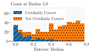
Figure 3: Certifiably correctness over median entropy.
