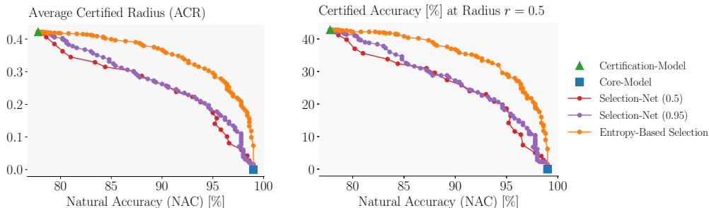
Figure 8: Comparing ACES with the entropy-based selection mechanism (orange) and selection networks (with \eta \in \{0.5, 0.95\} , red and purple) on CIFAR10 with respect to ACR (left) and certified accuracy at radius r = 0.5 (right) compared to natural accuracy. The certification network (ResNet110 trained with GAUSSIAN, \sigma = 0.25 ) and core-network (LaNet) are fixed.
