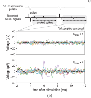
Fig. 8. (a) In vivo testing setup, (b) evoked neural signals after a stimulation pulse, (c) average evoked spikes per stimulation across charge modulation codes for 16 recording electrodes.
