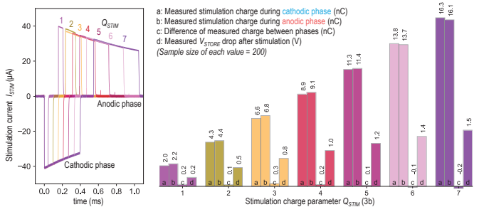
Fig. 7. Measured waveforms (left) and charge balancing characteristics (right) including integrated charge during each phase for different Q_{STIM} with a 100-kΩ electrode model.
