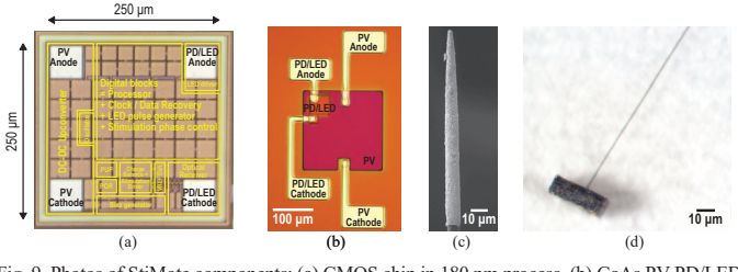
Fig. 9. Photos of StiMote components: (a) CMOS chip in 180 nm process, (b) GaAs PV-PD/LED cell, (c) PtIr-plated CF electrode, and (d) a dummy mote with stacked CMOS and GaAs layers.
