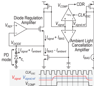
Fig. 3. TIA structure and its operation for optical receiver with ambient light cancellation.
