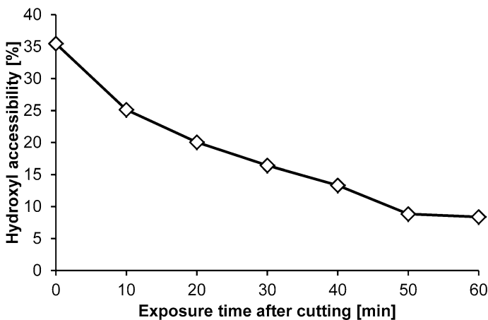
Fig. 2 Spectroscopically determined hydroxyl accessibility for one series of 15 \times 10 \times 3 mm 3 specimens of Norway spruce at different times of exposure to laboratory conditions after splitting in the middle
