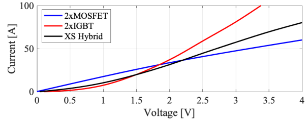
Fig. 2: IV characteristic of IGBTs, MOSFETs and XS hybrid semiconductors. The MOSFETs face lower internal resistances in the low load region compared to the IGBTs, leading to lower current losses. The behavior is reversed for the IGBTs, while the XS hybrid behaves like the average of the semiconductor coupling.
