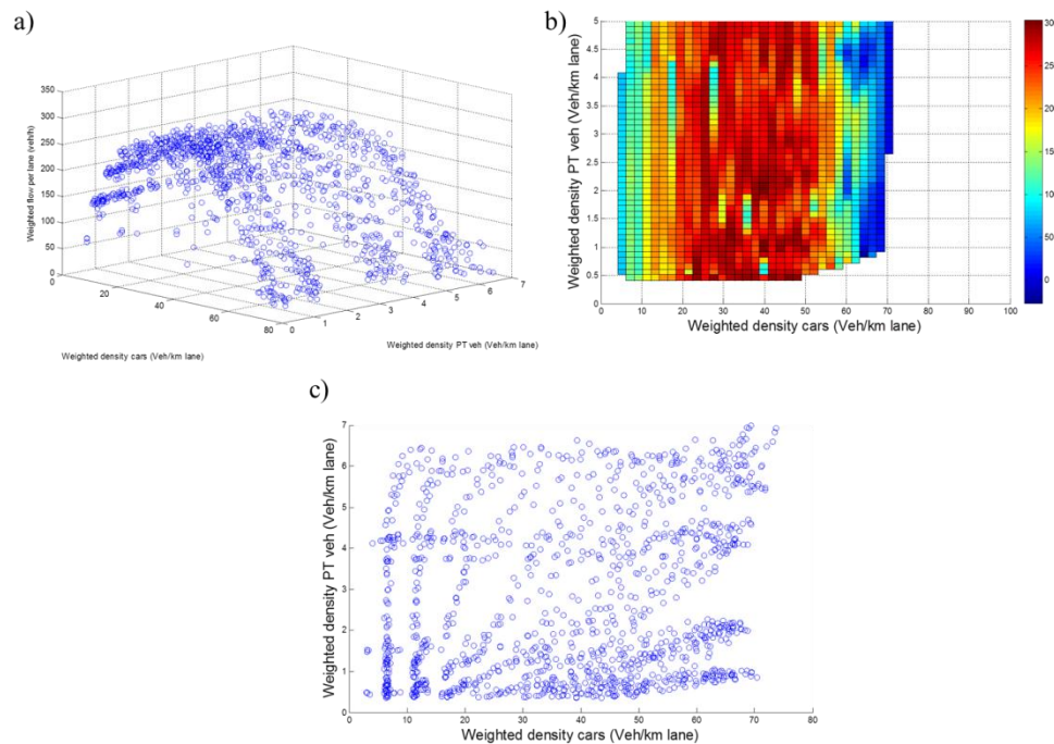
Figure 2. 3D-vMFD for the City of Zurich with dedicated lanes and without the priority signal system.
