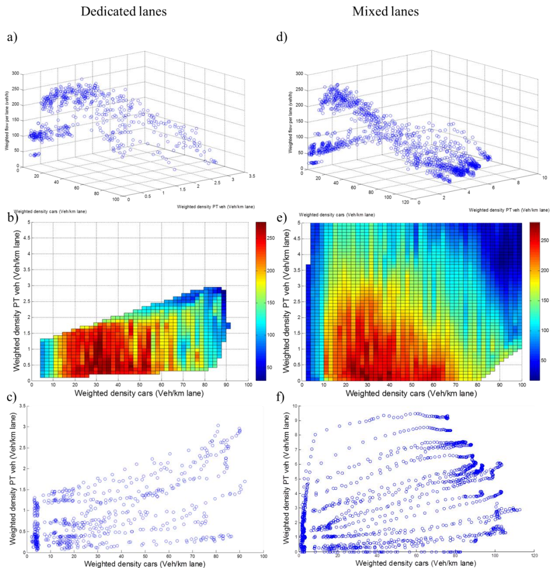
Figure 3. 3D-vMFD representations for San Francisco City: a-c) dedicated lanes, d-f) mixed lanes (Geroliminis et al., 2014).
