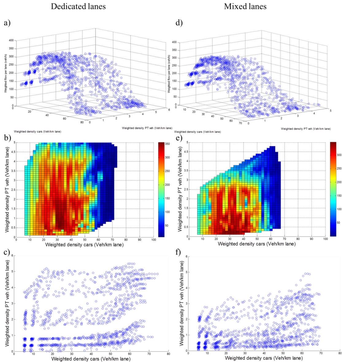
Figure 1. 3D-vMFD representations for the City of Zurich: a-c) dedicated lanes, d-f) mixed lanes.
