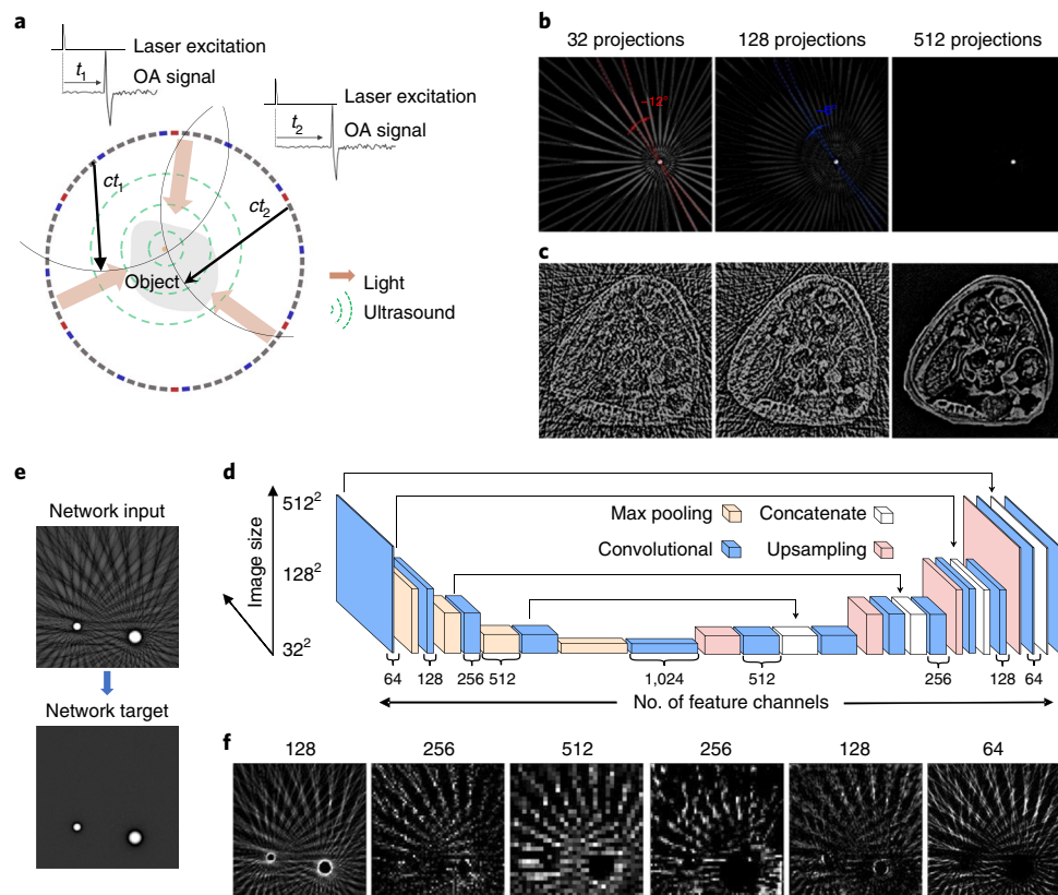
Fig. 1 | The deep convolutional neural network approach based on the U-Net architecture for artefact removal in OA imaging with undersampled data.
