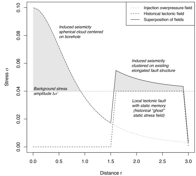
Figure 5. Sketch on how anisotropy and other types of heterogeneities can be implemented in the geometrical approach by adding a historical tectonic static stress field (ad hoc parameter values used for sake of simplicity). Here a past overloading field ( \sigma > \sigma_0^* + \Delta\sigma^* ) on a nearby fault would have been “planed” to the threshold \sigma_0^* + \Delta\sigma^* by temporal diffusion (Eq. 14), leaving only a “ghost” of that historical static stress field (for the homogeneous case, see Fig. 1a).
