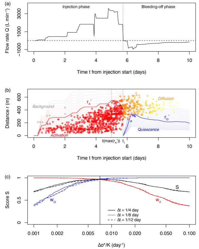
Figure 2. 2006 Basel EGS stimulation experiment data with activation and quiescence envelope fits: (a) flow rate Q(t) (digitised from Häring et al., 2008); (b) spatio-temporal distribution of relocated induced seismicity (Kraft and Deichmann, 2014) with r the distance from the borehole. The activation and quiescence envelopes r_A^*(t) and r_Q^*(t) are defined from Eq. (13) with parameters \widehat{\Delta \sigma^*} = 0.007 \text{ day}^{-1} (dark curves) and \Delta t = 1/4 day. The light curves represent the range \widehat{\Delta \sigma^*} \in [10^{-3}, 10^{-1}] \text{ day}^{-1} in 0.1 increments on the \log_{10} scale. Points represent the induced earthquakes; which colour indicates how they are declared. (c) Score S = (w_A + w_Q)/2 , with w_A and w_Q being the ratio of events of distance r \leq r_A^* and r \geq r_Q^* in the injection and bleeding-off phases, respectively. The vertical line represents \widehat{\Delta \sigma^*} = 0.007 \text{ day}^{-1} .
