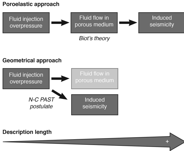
Figure 4. Description length defined as the count of physical steps required to describe induced seismicity, in poroelasticity and in the newly proposed geometrical approach. In the latter, Biot’s theory is entirely bypassed.
