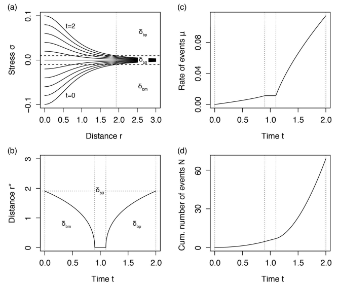
Figure 1. Seismicity spatio-temporal behaviour described by the N-C PAST static stress model (tectonic case; Mignan, 2012): (a) spatio-temporal evolution of the stress field \sigma(r, t) generated by constant stress accumulation \dot{\tau} on a fault located at r = 0 (Eq. 1). Background, quiescence, and activation seismicity regimes are described by densities of events \delta_{b0} , \delta_{bm} , and \delta_{bp} for |\sigma| \leq \sigma_0^* \pm \Delta\sigma^* , \sigma < \sigma_0^* - \Delta\sigma^* , and \sigma > \sigma_0^* + \Delta\sigma^* , respectively; (b) temporal evolution of quiescence and activation envelopes r^*(t) , with \sigma(r^*) = \sigma_0^* \pm \Delta\sigma^* (Eq. 2); (c) rate of events \mu(t) in a disc of constant radius \max(r^*) (Eq. 3); (d) cumulative number of events N(t) (Eq. 4) of power law form (Eq. 5), with t_0 = 0 , t_{mid} = 1 , t_f = 2 , h = 1 , \dot{\tau} = 0.1 , \sigma_0^* = 0 , \Delta\sigma^* = 10^{-2} , \delta_{bm} = 0.001 , \delta_{b0} = 0.1 , \delta_{bp} = 1 , n = 3 , k = \pi , d = 2 , \Delta t = 0.01 .
