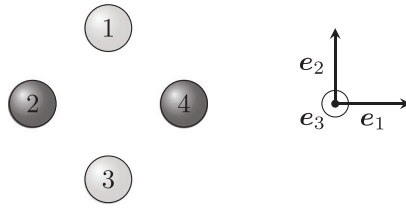
FIGURE 5 A quadrimer constituted of four resonators rotationally invariant around the axis e_3 . The alternate colors emphasize the existence of the mode [1 \ -1 \ 1 \ -1]^T
