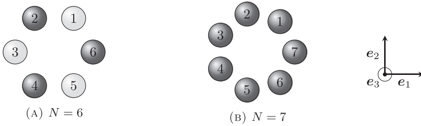
FIGURE 2 Chains of, respectively (three-dimensional), six and seven spherical resonators rotationally invariant around the axis e_3 . The rotational symmetry entails the invariance of the geometry by the permutation group generated by the N -cycle \sigma = (0 \dots N - 1) . The alternate colors visible in Figure 2A with N = 6 illustrates the fact that the sign changing vector ((-1)^i)_{1 \leq i \leq N} is an eigenvector of the capacitance matrix C when N is even
