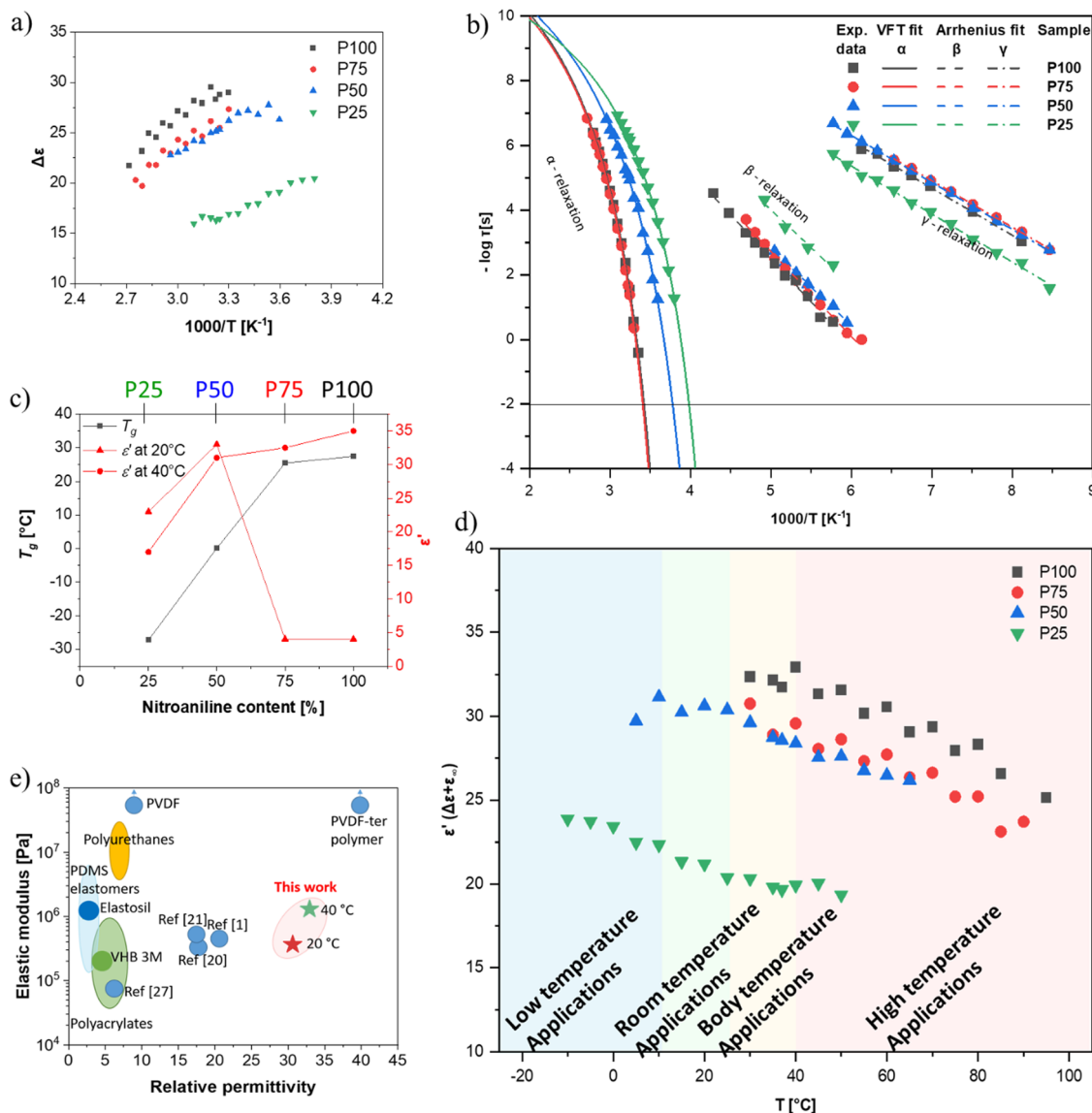
Fig. 3 (a) Relaxation strength ( \Delta\epsilon ) of the dipoles extracted from the HN-fit at different temperatures and Arrhenius plot of the four polymers with VFT-fit for the \alpha -relaxation and Arrhenius-fits for the \beta and \gamma (c) dependency of T_g and permittivity with varying nitroaniline and cyanopropyl content and temperature. (d) Absolute permittivity of the different polymers at different temperatures extracted from the relaxation strength ( \Delta\epsilon ) and background permittivity ( \epsilon_\infty ; values taken at -150^\circ\text{C} and 10^6 \text{ Hz} ). (e) Comparison of the relative permittivity and material elastic modulus with materials from literature.
