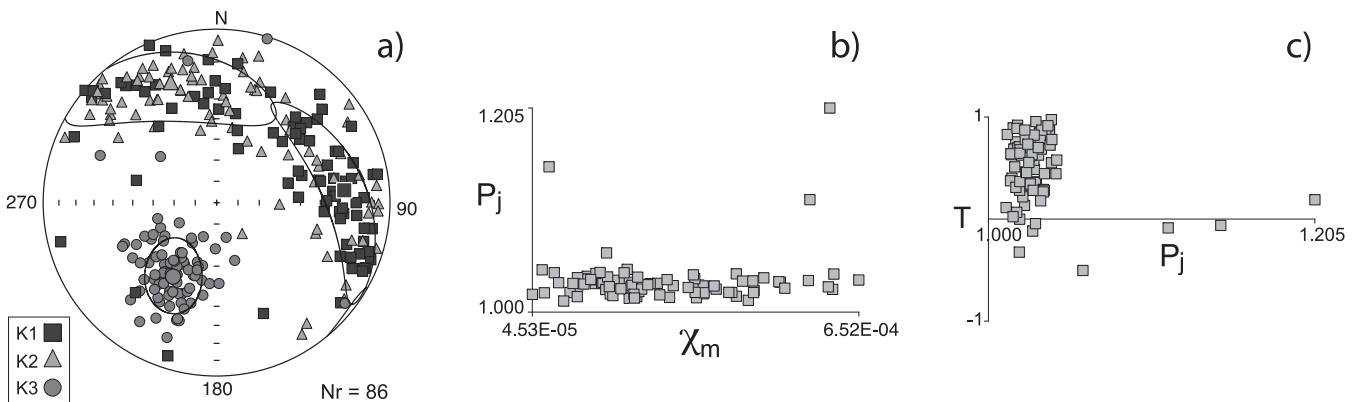
Figure 9. (a) Anisotropy of susceptibility for all specimens. Squares represent maximum k_1 , triangles intermediate k_2 and circles minimum k_3 susceptibilities. Larger symbols are averages for the principal axes, and ellipses are 95 per cent confidence intervals. Data are plotted on an equal-area, lower hemisphere projection in geographic coordinates. (b) Anisotropy degree P_j versus average bulk susceptibility \chi_m . (c) Shape parameter T versus P_j .
