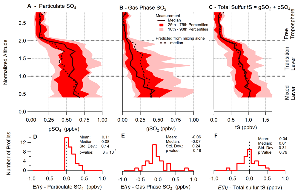
Figure 12. Altitude-normalized profiles of (a) particulate sulfate, (b) gas-phase \text{SO}_2 , and (c) total sulfur \text{tS} . The shaded regions show the interdecile range (light) and the interquartile range (medium), and the solid lines are the median (dark). The dashed line shows the median value expected from mixing alone. Histograms of the transition layer enhancement ( E(h) ) and the results of the t test for (d) particulate sulfate, (e) \text{SO}_2 , and (f) total sulfur are shown.
