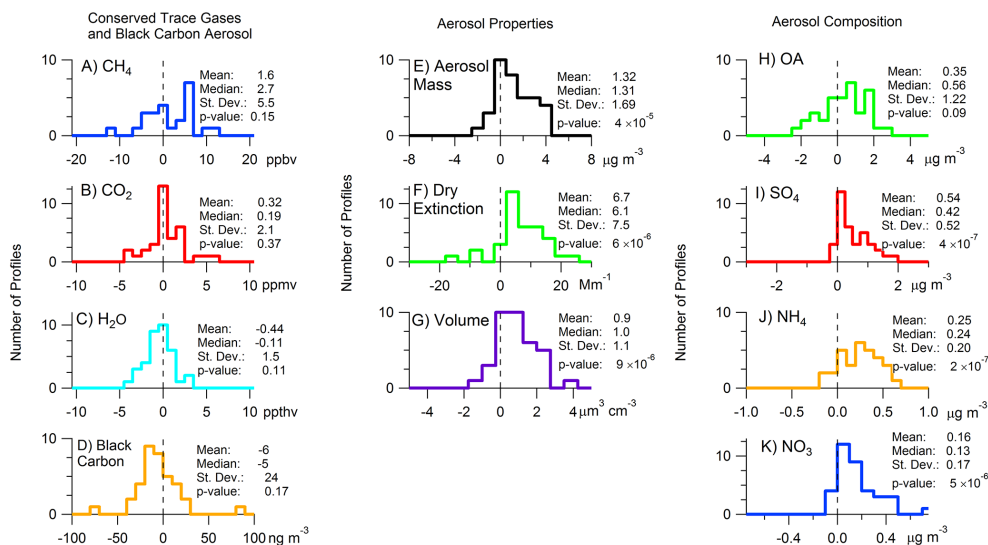
Figure 11. Histograms of the transition layer enhancement ( E(h) – see Eq. 4) for several trace gases and aerosol properties. The first column shows conserved species and black carbon: (a) \text{CH}_4 , (b) \text{CO}_2 , (c) \text{H}_2\text{O} , and (d) black carbon mass. The second column shows the aerosol extensive properties: (e) aerosol mass, (f) dry extinction, and (g) aerosol volume. The third column shows the aerosol composition: (h) OA, (i) \text{SO}_4 , (j) \text{NH}_4 , and (k) \text{NO}_3 . The Student's t test and resulting p value (noted in each histogram) were used to test whether the mean of each distribution was statistically different from 0.
