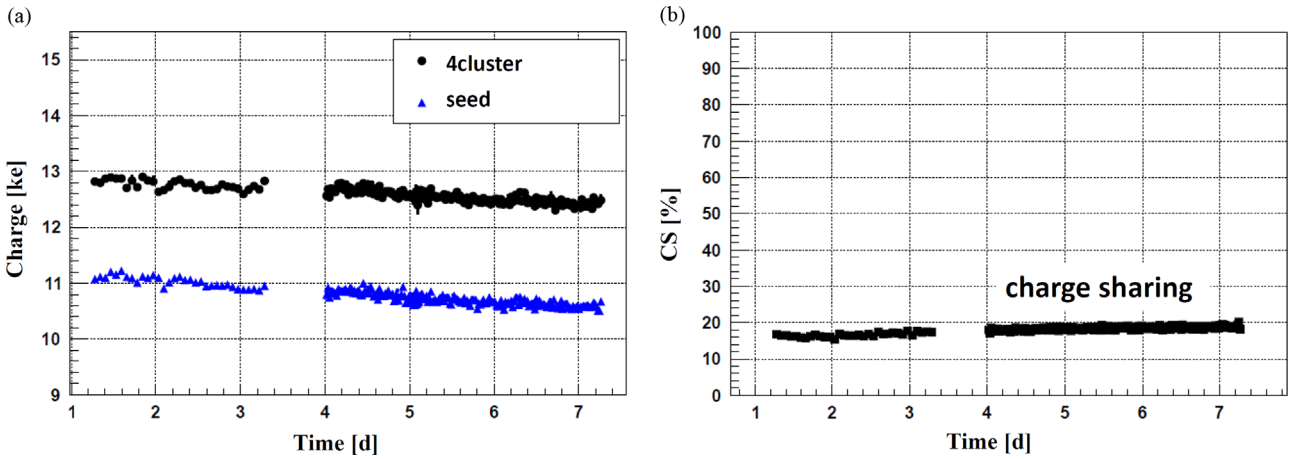
Fig. 10. (a) Median of the PH(4-cluster) and PH(seed) distributions for the FZ p -stop sensor irradiated by 15 \times 10^{14} n_{eq}/\text{cm}^2 24 GeV/c protons and 6 \times 10^{14} n_{eq}/\text{cm}^2 reactor neutrons as a function of the measurement time, during which the dose in the SiO 2 from the \beta source increased from 0 to 375 Gy(SiO 2 ). The applied voltage was 1000 V. (b) The corresponding time dependence for CS.
